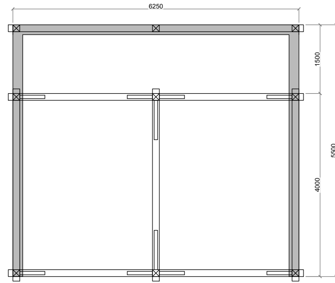
Frame Plan
